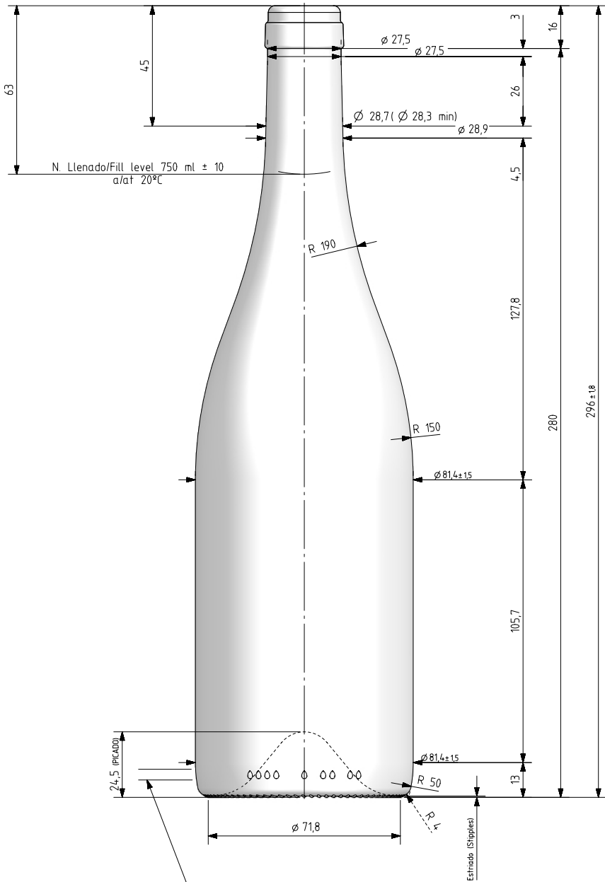
VISTA FRONTAL (FRONT VIEW)
